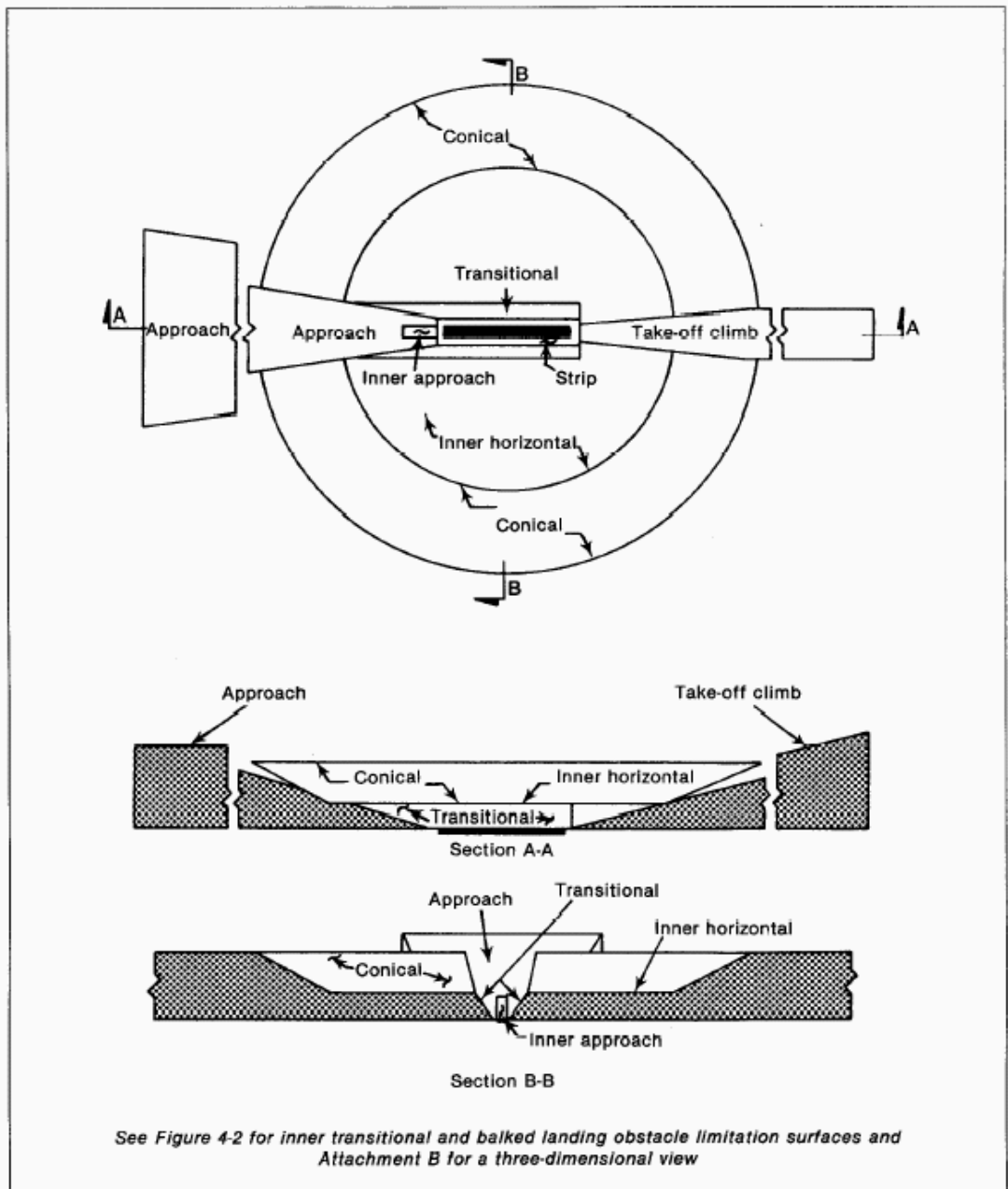
Figure 4-1. Obstacle limitation surfaces
